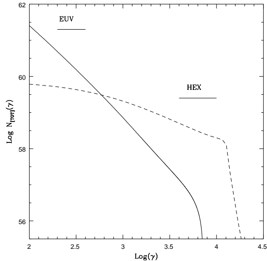
Figure 3: Plot of the energy distribution of the relativistic electron populations in the Coma cluster. The dashed line represents the main electron population, integrated over the cluster volume, injected during the first phase and reaccelerated during the second phase . The solid line refers to the additional IC electron population injected by the radio galaxy NGC 4869. The typical energies of the electrons emitting via IC in the hard X-ray band (HEX) and in the EUV band are also indicated.
